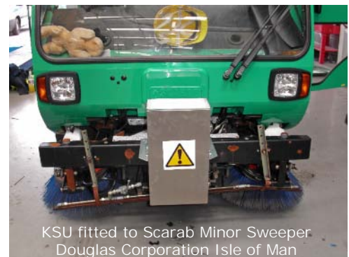
KSU Rear Mounted Spray Arm fitted to Johnson Sweeper
